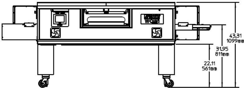
PS670-2 Double Oven with 15\" (381mm) leg extensions
