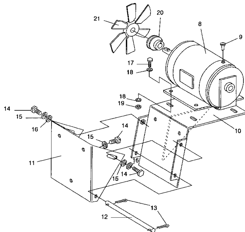
FIGURE 6-8 MACHINERY COMPARTMENT FIGURE 6-8 COMPARTIMENT DU MÉCANISME
