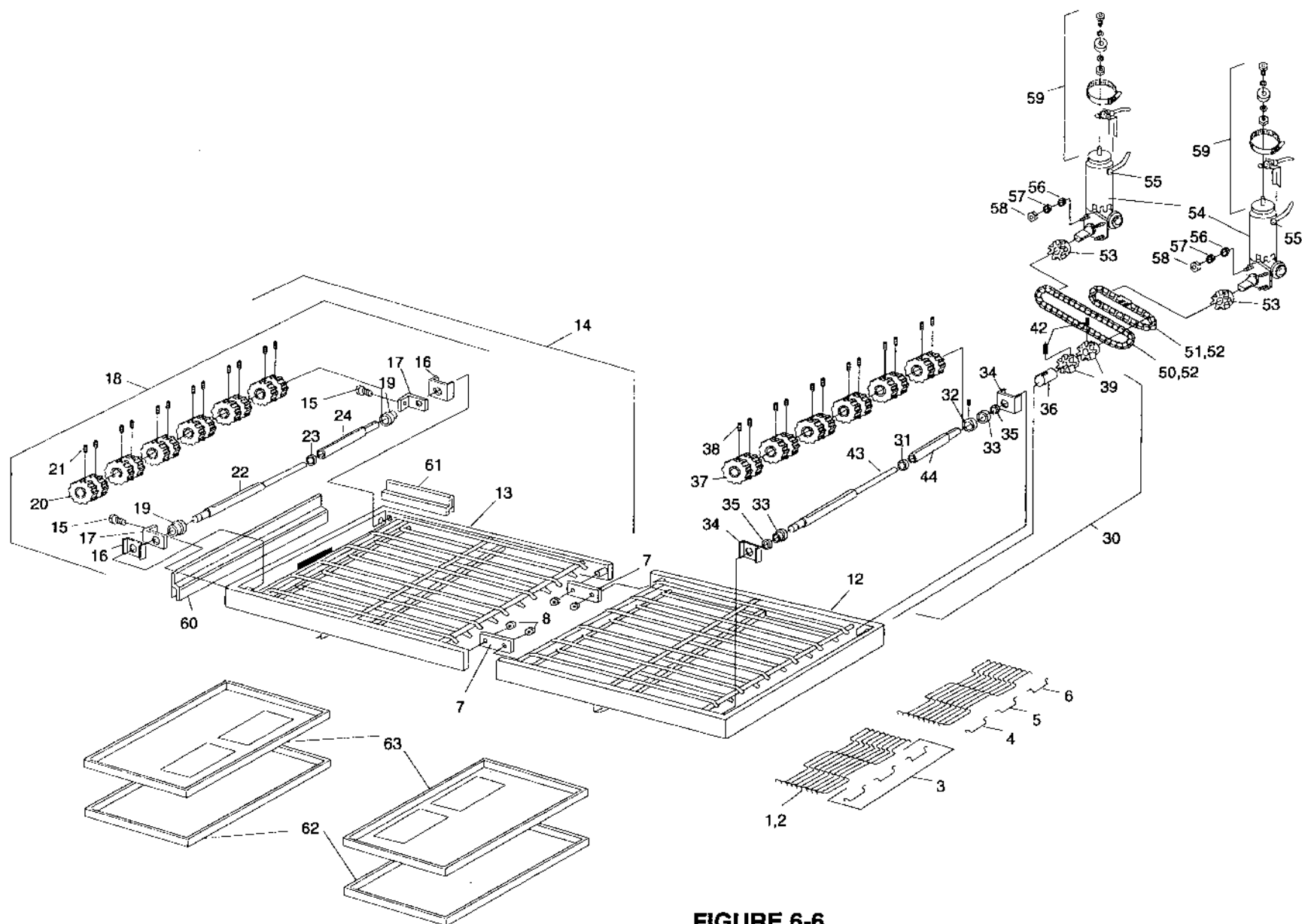
FIGURE 6-6 SPLIT BELT CONVEYOR FIGURE 6-6 CONVOYEUR À TAPIS JUMEAUX
