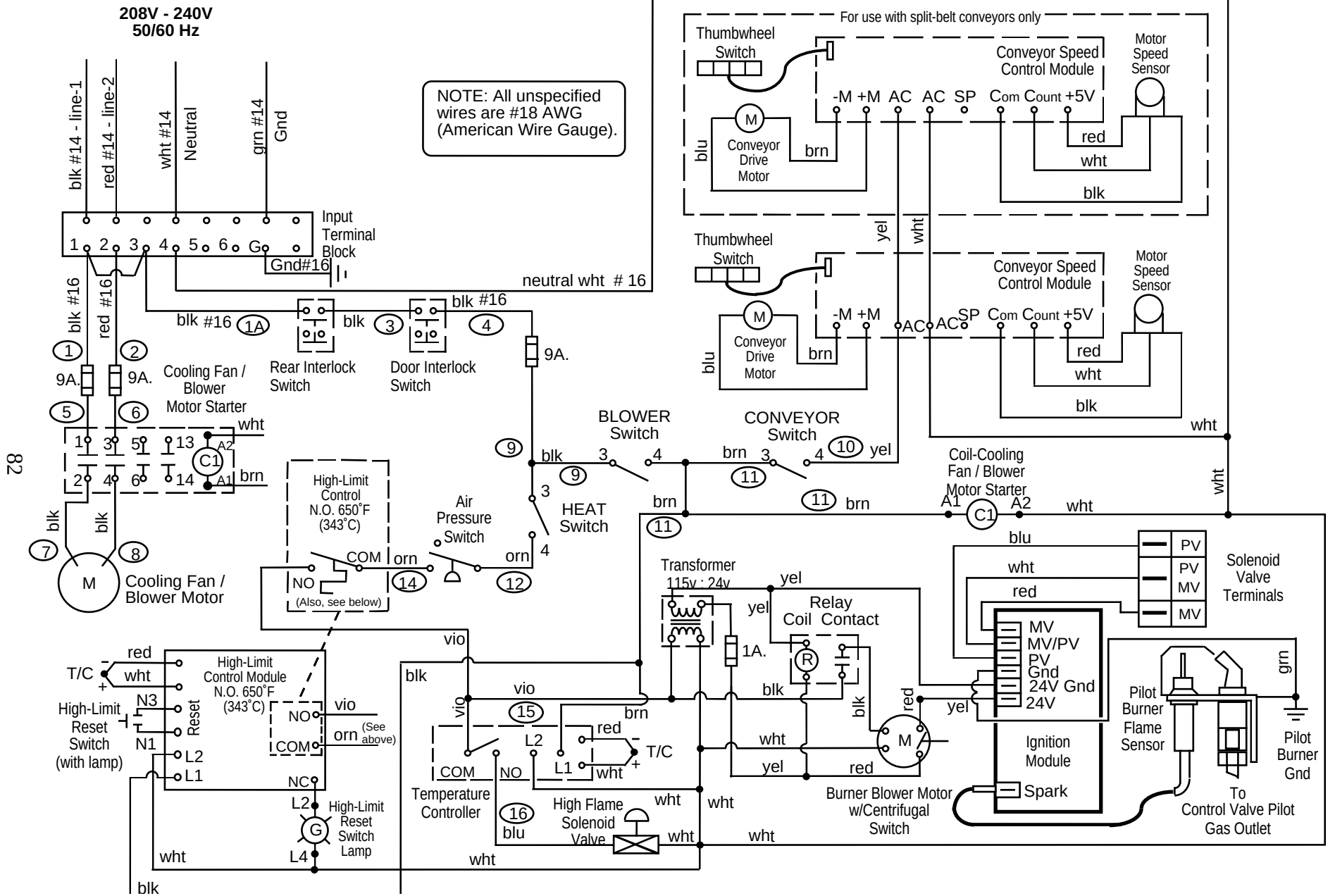
PS200VL-SERIES GAS OVEN SCHEMATIC: 208V- 240V Blower Motor, 50/60Hz, 1 Ph, 4.1 A. Draw, 3-Pole, 4-Wire (2 powered, 1 neutral, 1 grd), 120V Control Circuit
