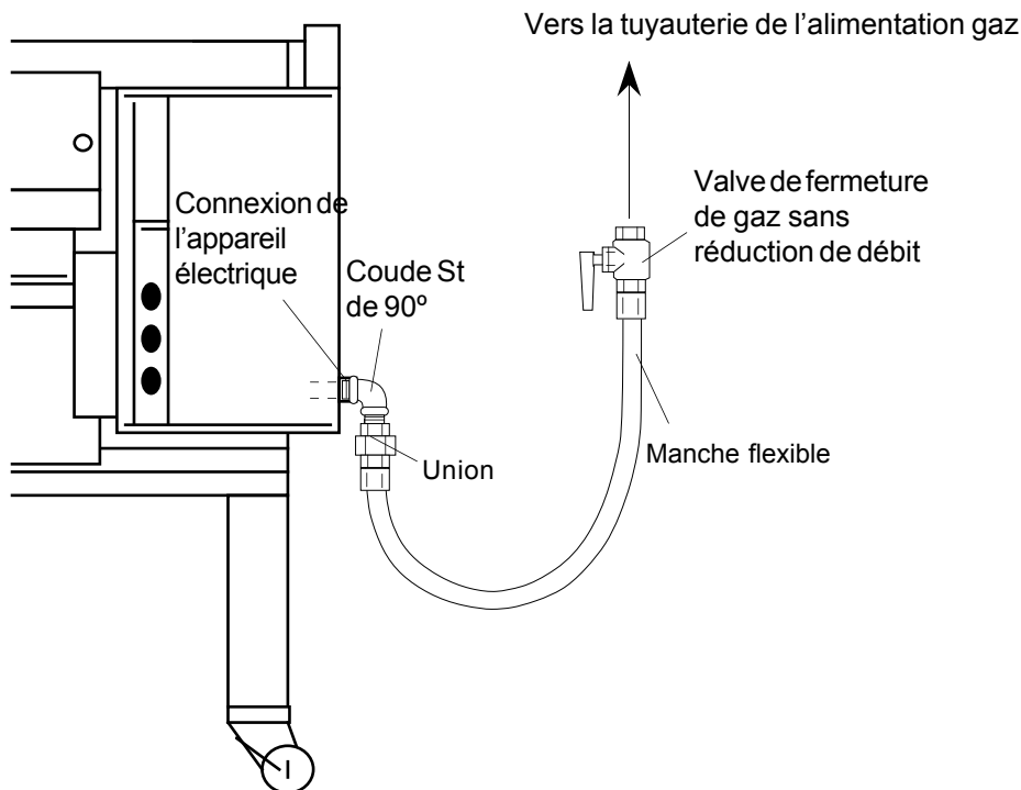
Figure 2-13. Installation du manche flexible
