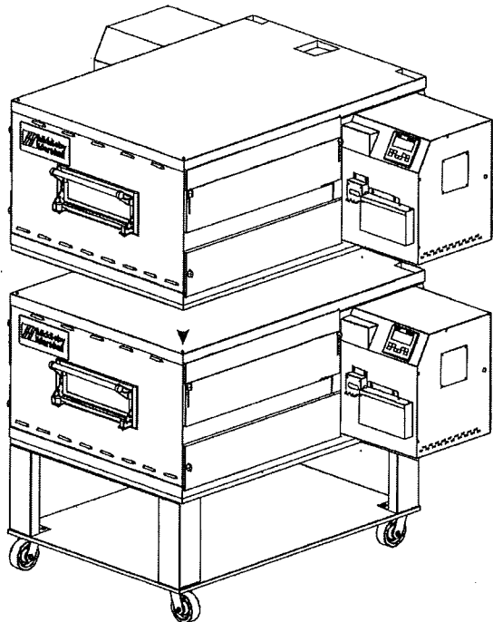
Figure 2-9. Stacking
