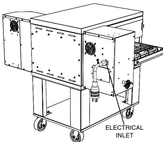
Figure 2-11. Junction Connection Box
