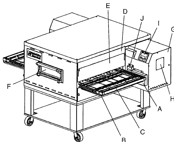
Figure 1-1. Oven Components
