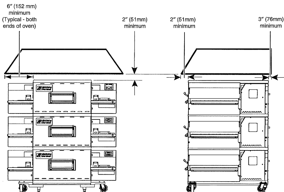
Figure 2-5. Ventilation System
