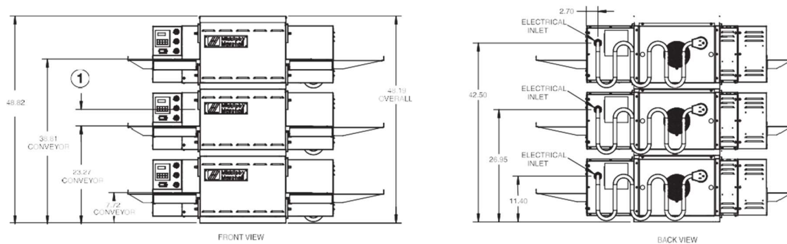
Figure 2-7. MODEL PS520 TRIPLE OVEN DIMENSIONS
