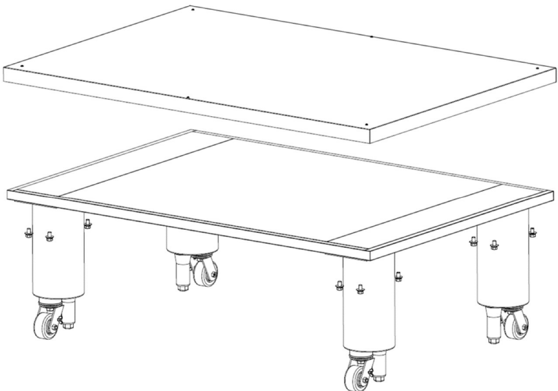
View of X70G/X55G/X55GWB TRIPLE OVEN BASE/TOP KIT
