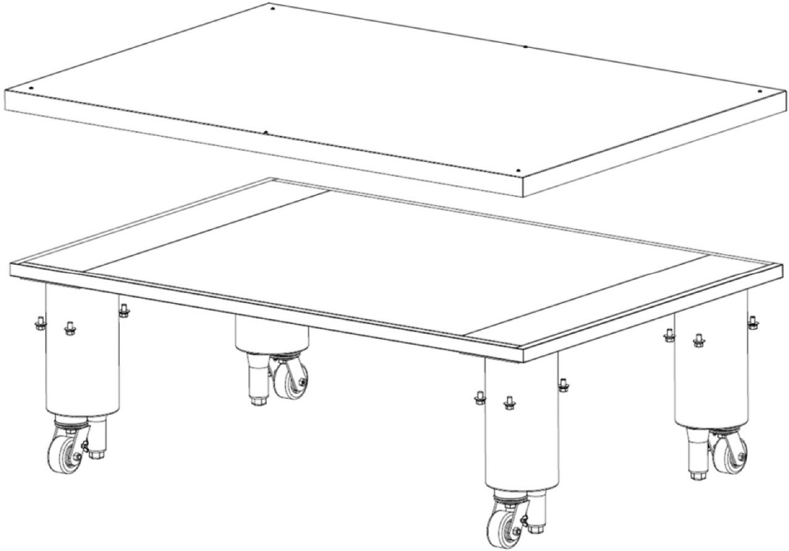
View of X70G/X55G OVEN BASE/TOP KIT with 19" LEGS
