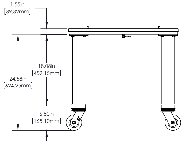
PS520 18" Oven Cart Front View
