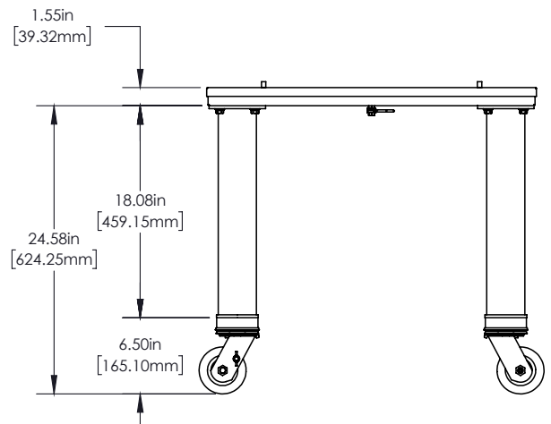
X26 Oven Cart Front View
