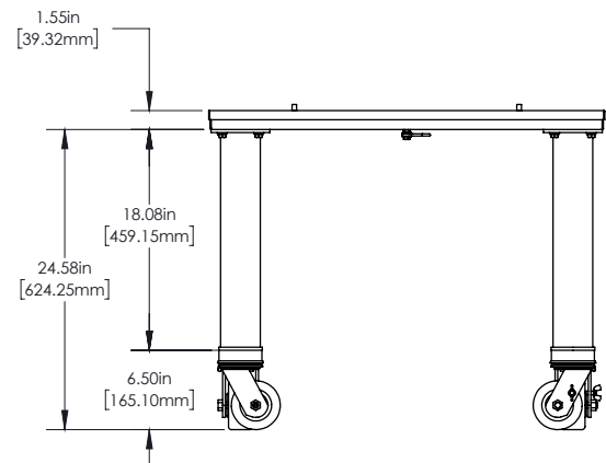
X20 Oven Cart Front View
